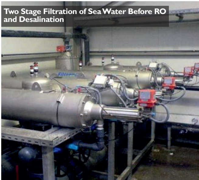
Two Stage Filtration of Sea Water Before RO and Desalination
